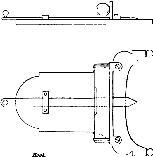
Laryard and Handle.
