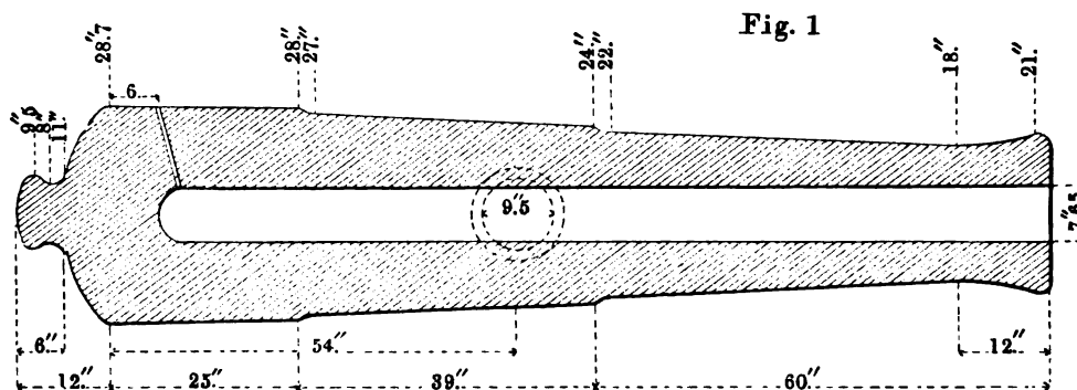
Russian 56-Pdr. Gun
